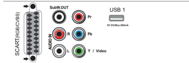
Connections Bottom
